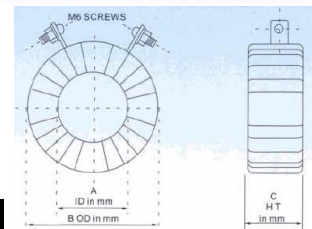
GENERAL VIEW OF THE PR &amp; MR SERIES CT
